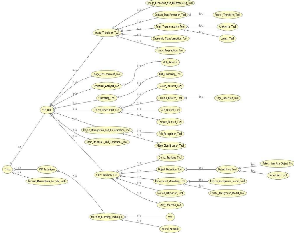
Figure 6: Main concepts of the Capability Ontology.
