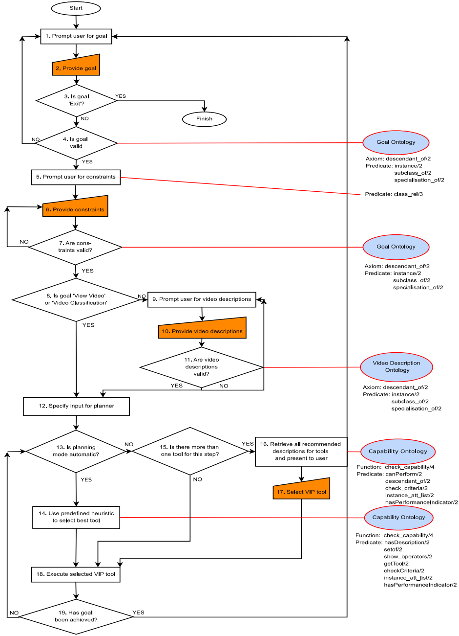
Figure 7: Flowchart of the workflow enactor's interaction with the user annotated with ontology use. Shaded processes denote user-provided input.
